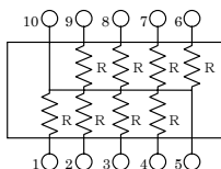
並列回路 / Bussed Circuit TSN1F
