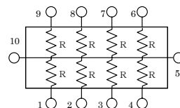
並列回路 / Bussed Circuit TSN9M
