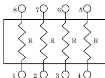
独立回路 / Isolated Circuit TSN2N,3N,8N
