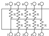
並列回路 / Bussed Circuit TSN1C
